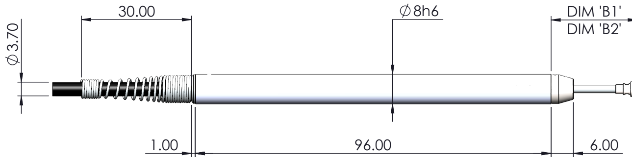
AXIAL CABLE OUTLET - AW/5/S(H)
