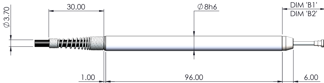
AXIAL CABLE OUTLET - DW/10/S
