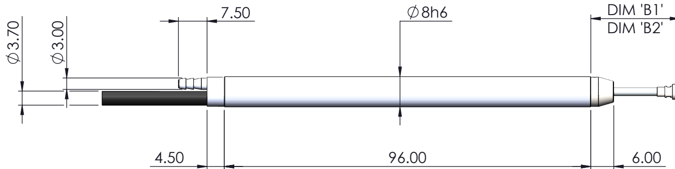
AXIAL CABLE OUTLET - DW/10/V
